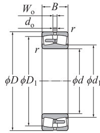
Cylindrical bore
