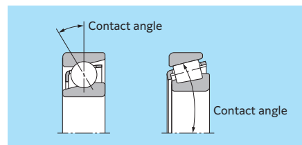
Fig. 1.3 Contact angle
